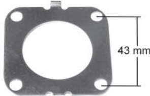
234573 Servicing A14VI48, SG12B020, -040, -045, SG15L026, SG15S019, -024 O.D. 57 x 57 mm I.D. 37 mm Bearing plate
