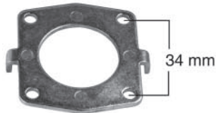
232060 Std pkg 5 Servicing A115i I.D. 28 mm Bearing plate
