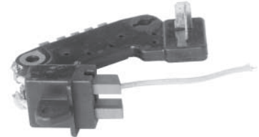
132089 Replacing L135N-13301, 23135-B9800 Servicing LR135-44, LR138-01, -72R, LR150-35, -36, -51, -53, -58 12 V. Complete w/ brushes
