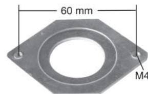
234574 Servicing A13N1M, -2M, -35M, -147M, -148M, -149M, -186M, -259M, A14N104, -138, -139, -172, -205 O.D. 72 x 53 mm Bearing plate
