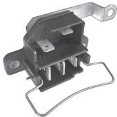
135881 Std pkg 5 Servicing 633 210 59 Terminal block Terminal lock: Cargo 139963
