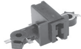
132426 Replacing L150-43303, 23135-V6600 Servicing LR140-130P, -402, -406, -408, -410, -410B, -410BA, -410F, -410G, -411 -411B, -411BA, -411F, -411G, -415, -415B -419T, -421, -422E, -422T, -423, -423F 12/24 V. Complete w/ brushes
