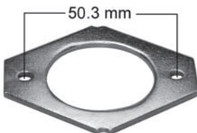
231864 Servicing A13N181 I.D. 35.5 mm Bearing plate
