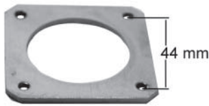
233440 Servicing A14VI... O.D. 57 x 57 mm I.D. 40.2 mm Bearing plate
