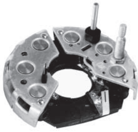
133998 HD Replacing 1127 320 914 Servicing 0120 488 186, -187
